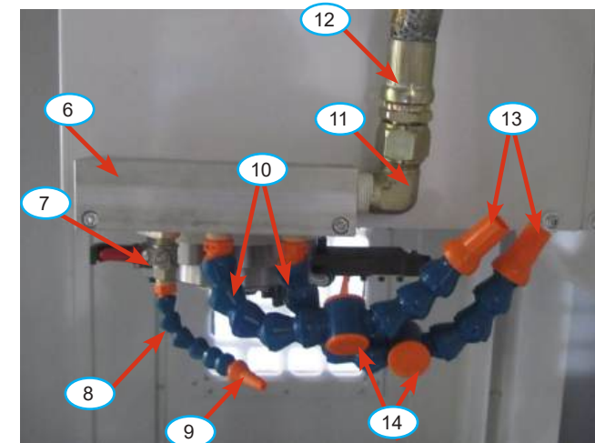
MACHINE ENCLOSURE
