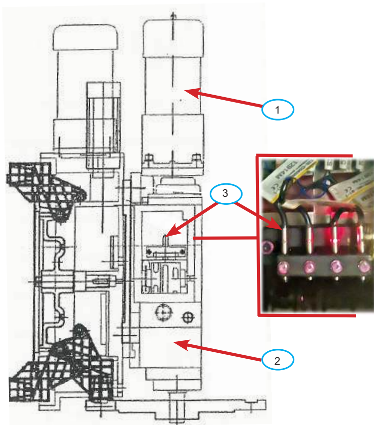
Gearbox Assembly
