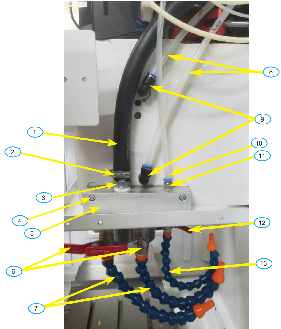
HEAD PLUMBING
