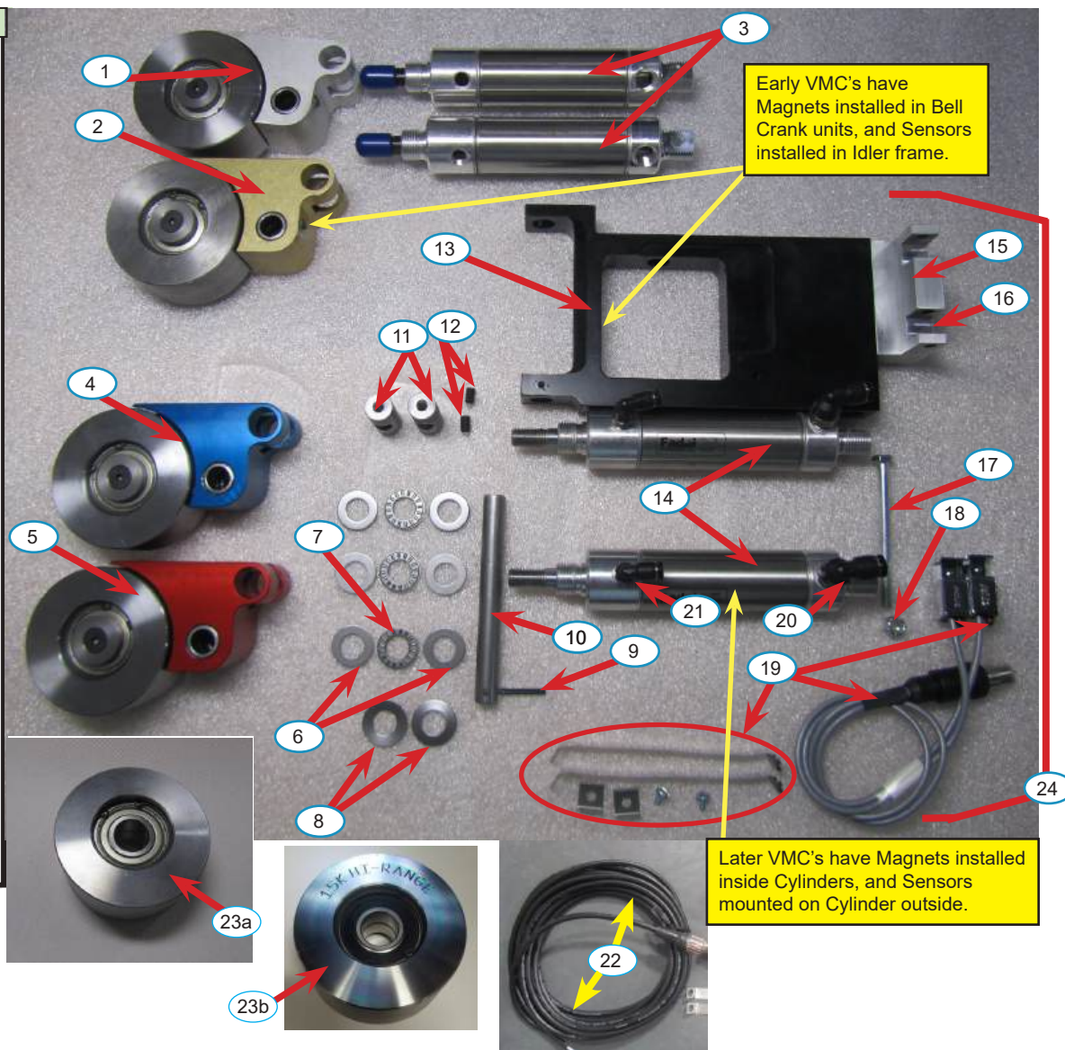
IDLER ASSEMBLY
