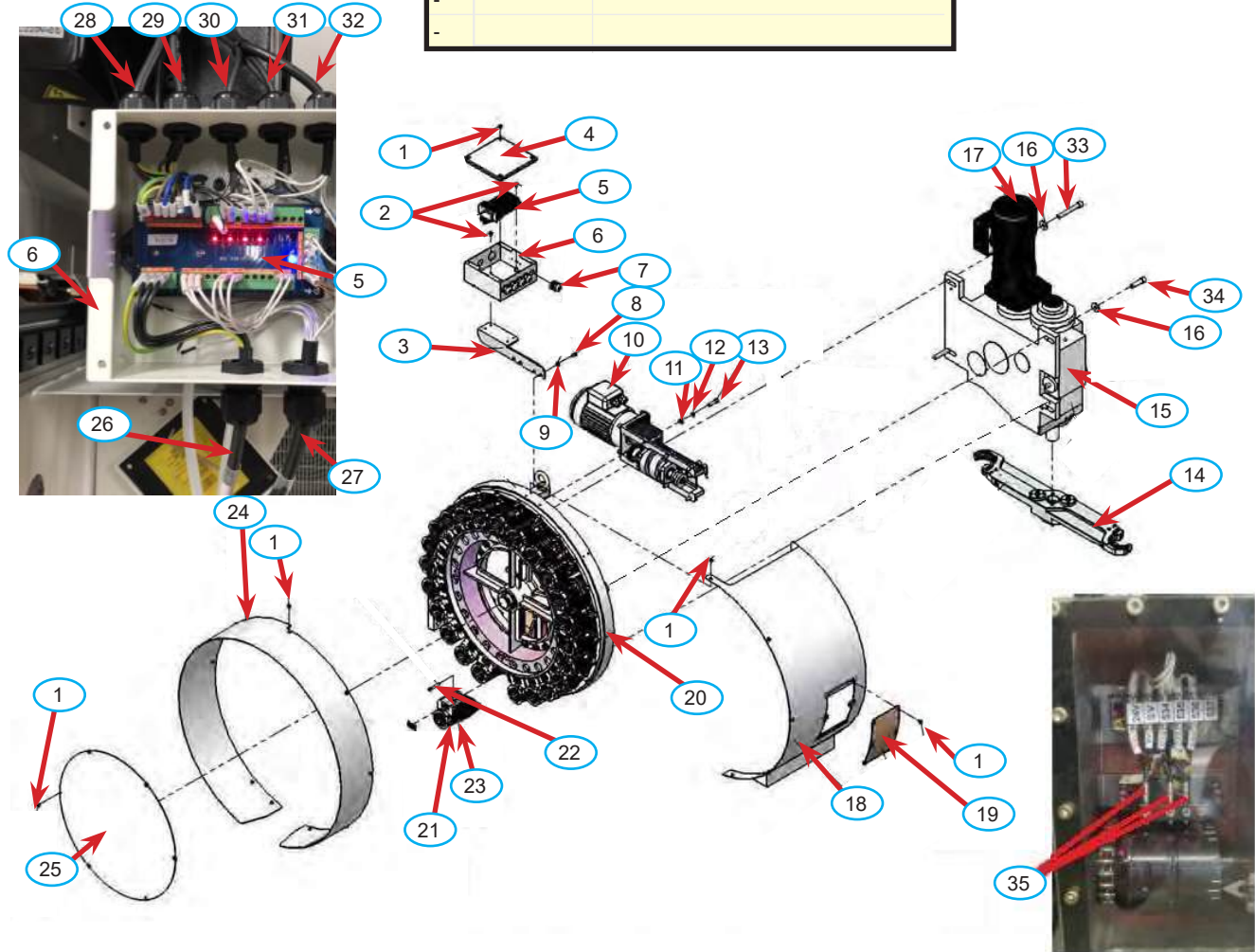
DUAL ARM TOOLCHANGER 24
