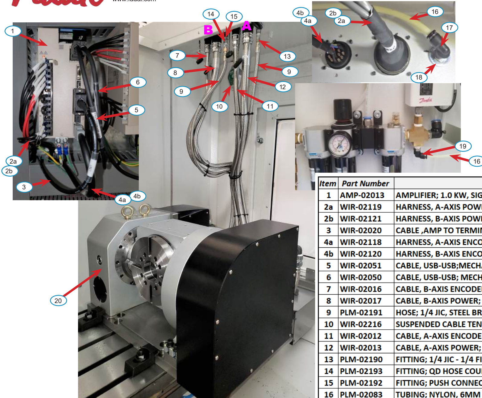
8" TILTING ROTARY
