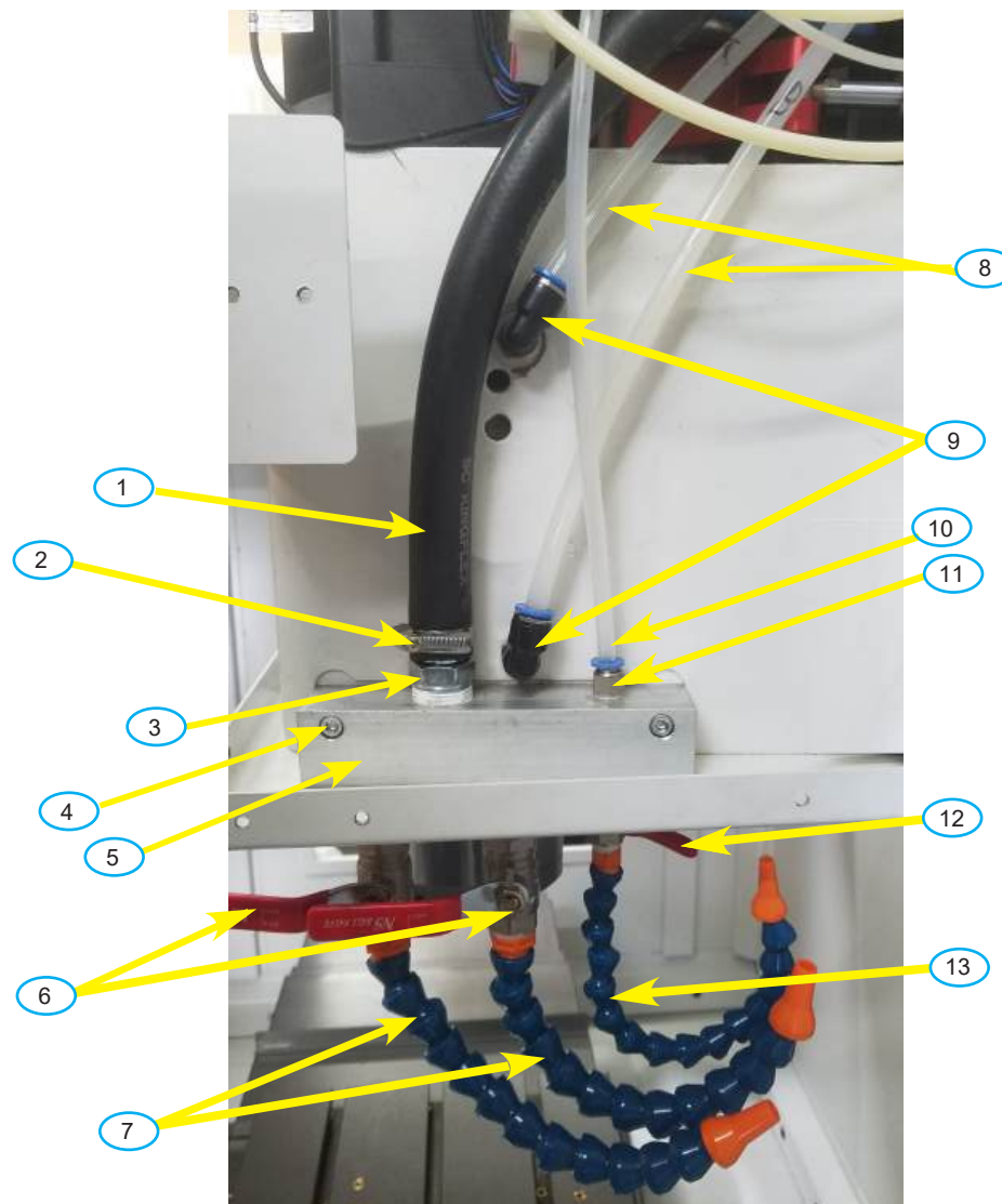
HEAD PLUMBING
