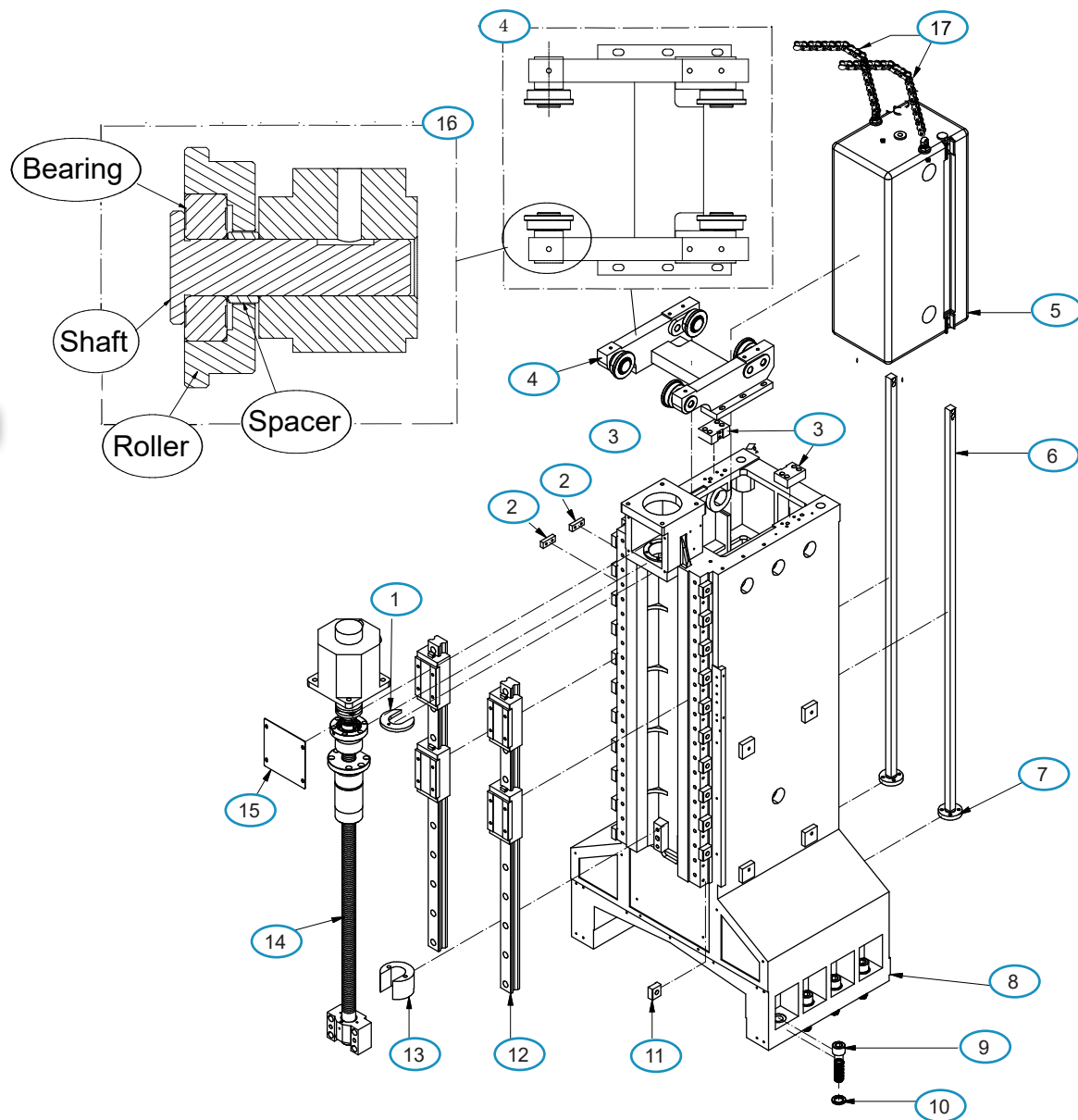
COLUMN AND COUNTERWEIGHT - STANDARD Z
