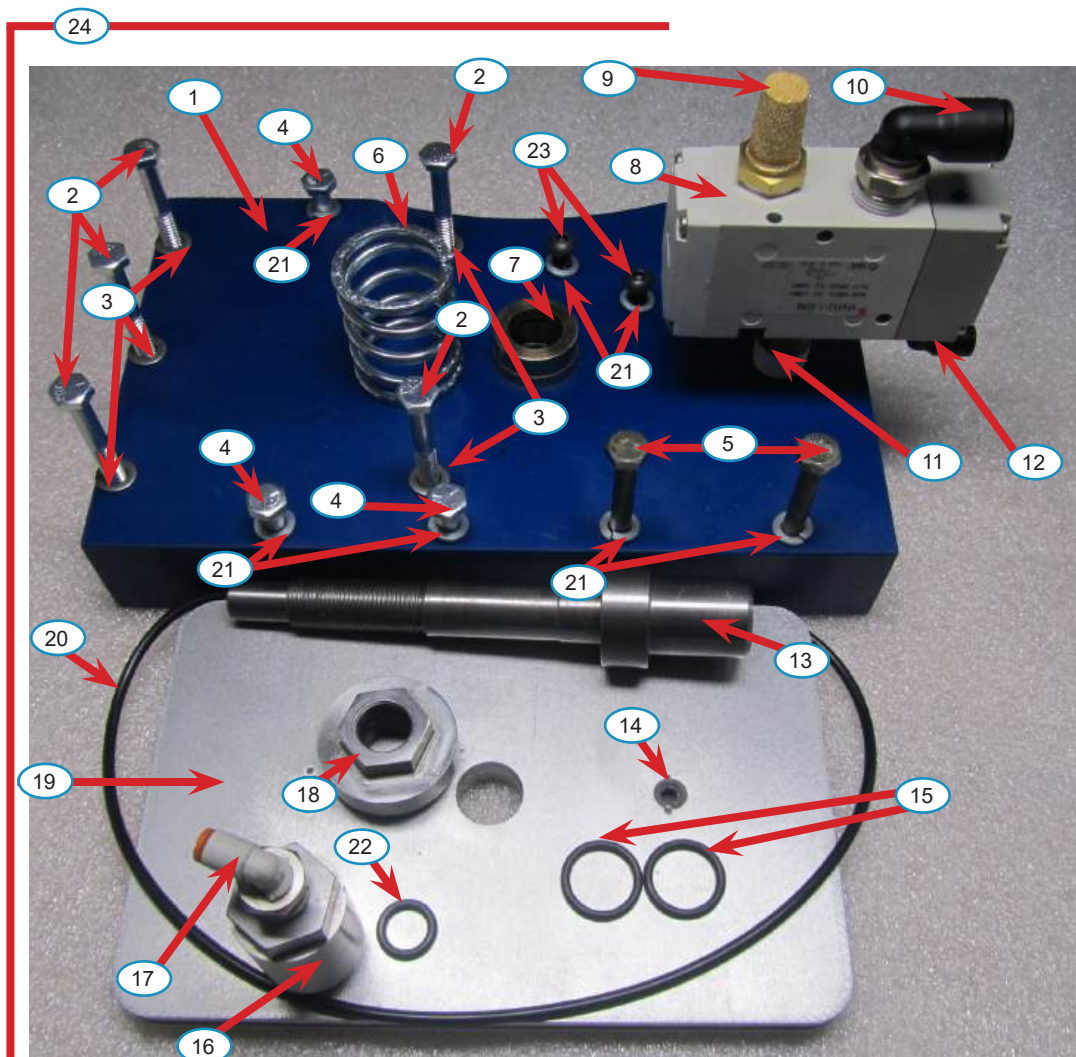
DRAWBAR CYLINDER-UPPER THREADED PISTON
