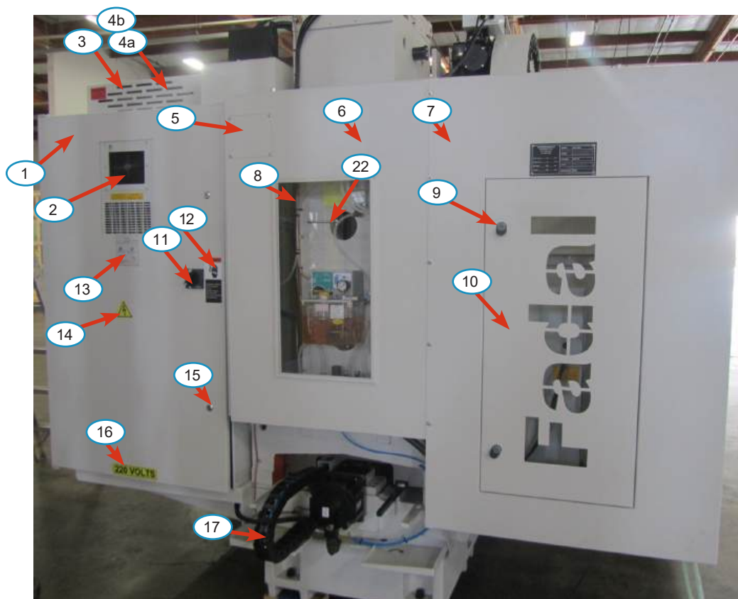
ENCLOSURE - REAR / LEFT SIDE
