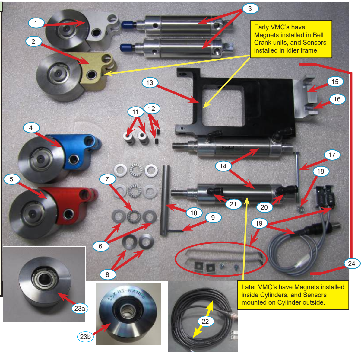
IDLER ASSEMBLY
