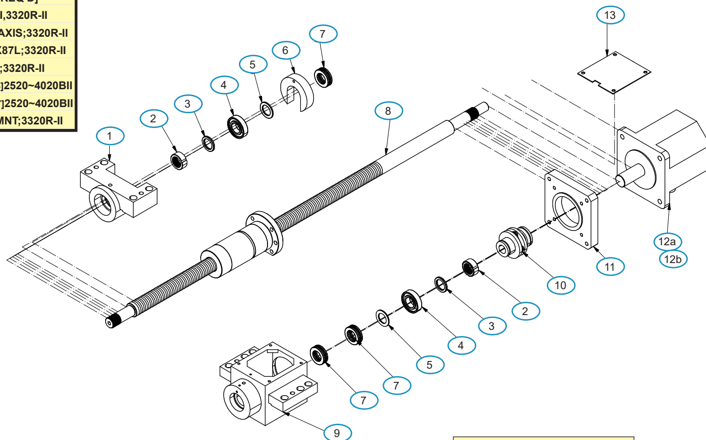
Y-AXIS BALLSCREW
