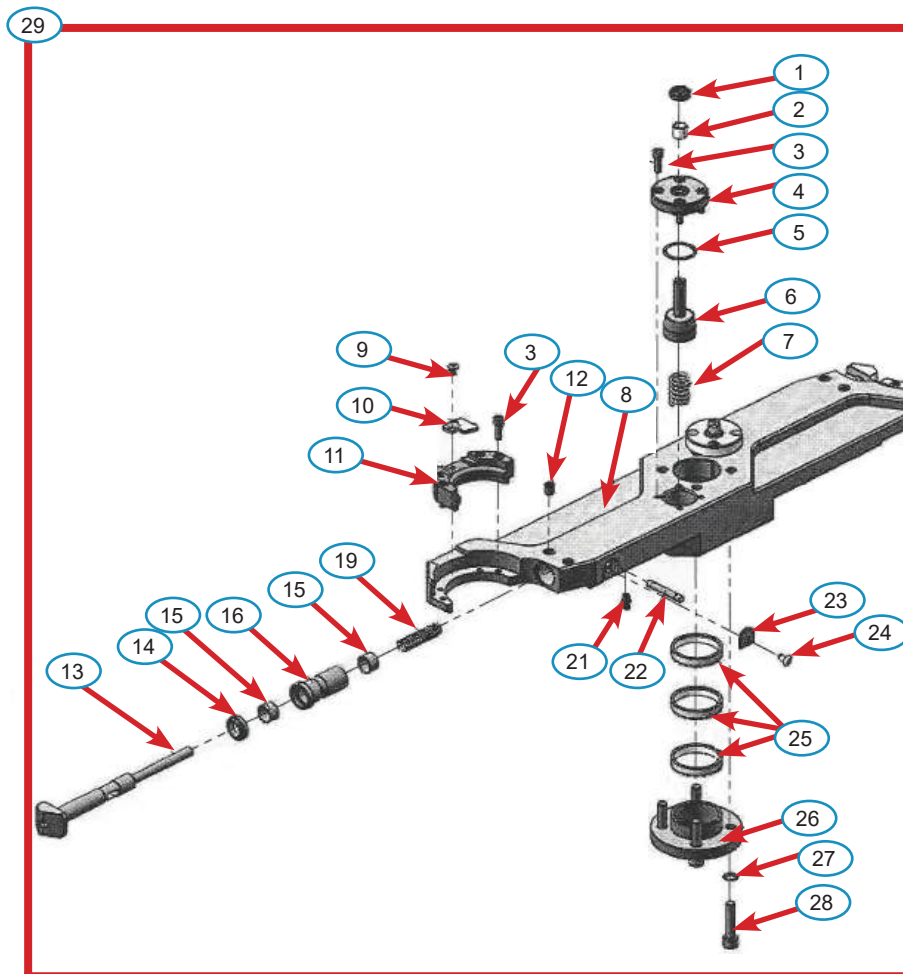
DUAL ARM TOOL CHANGER 24/30
