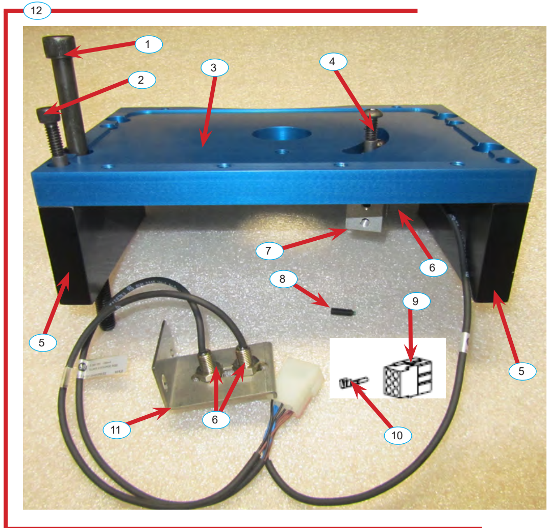
ORIENTATION BRIDGE
