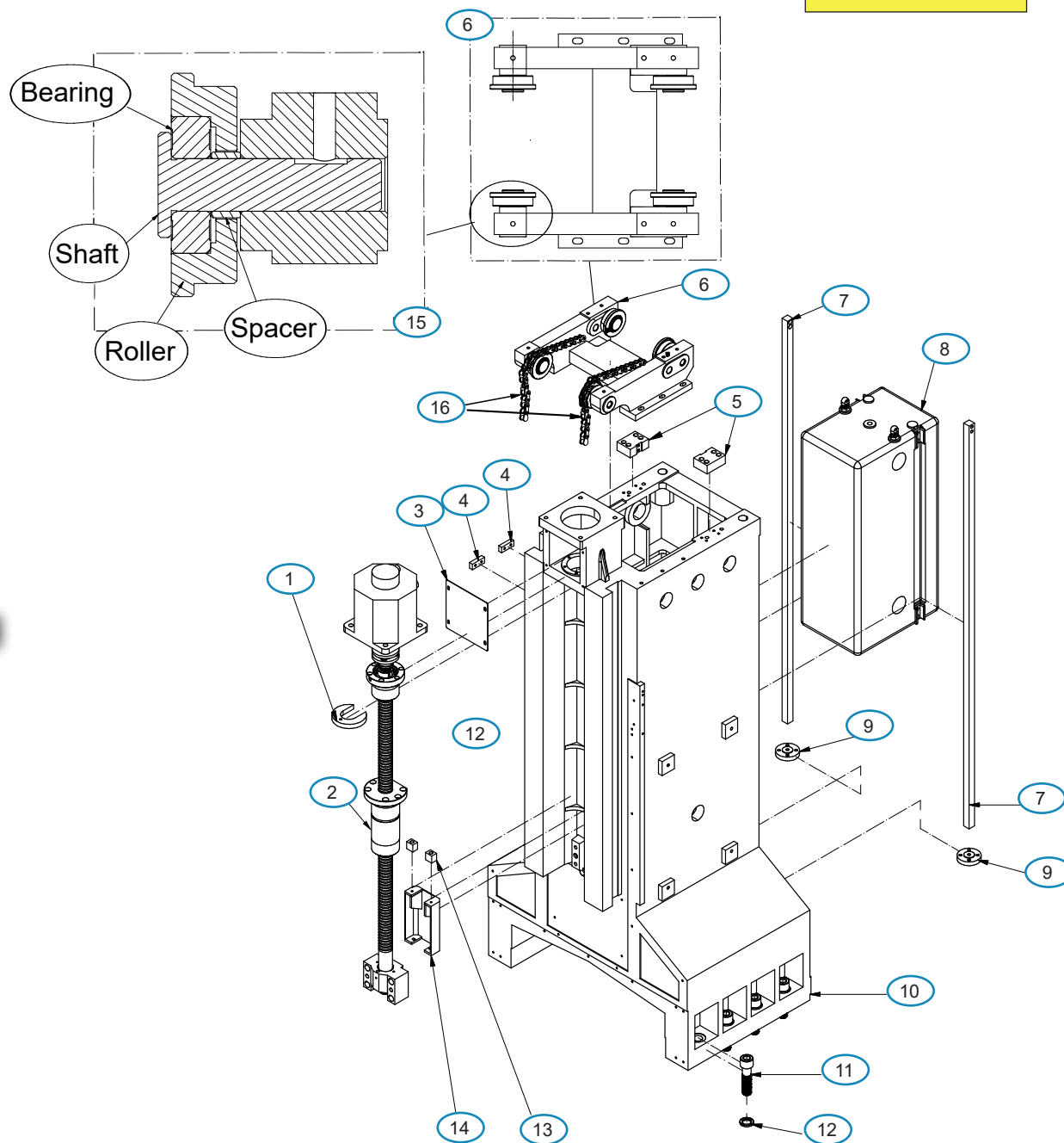
COLUMN AND COUNTERWEIGHT - STANDARD Z
