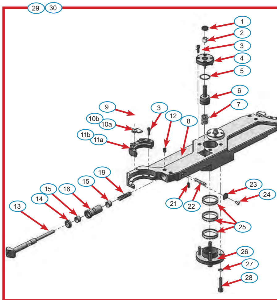
DUAL ARM TOOLCHANGER 24/30/40
