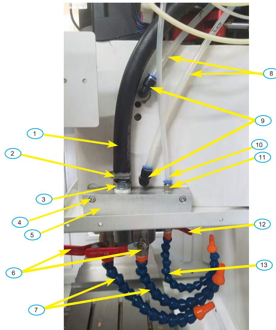
HEAD PLUMBING
