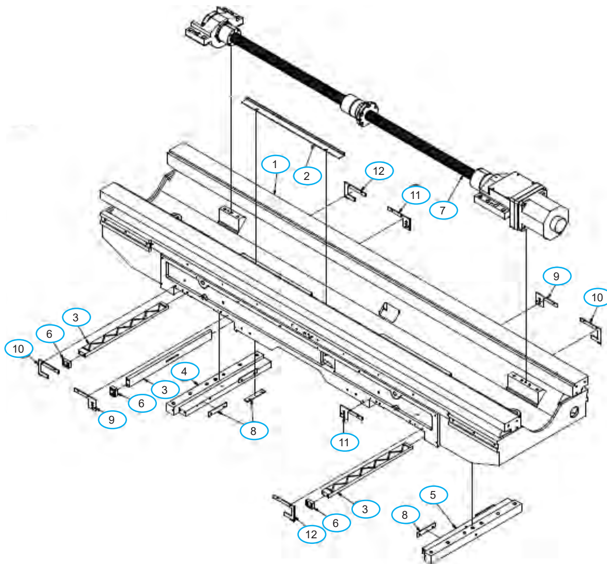
SADDLE CASTING
