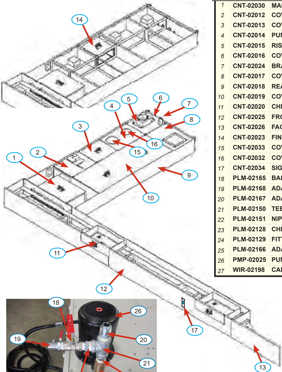
COOLANT TANK ASSEMBLY
