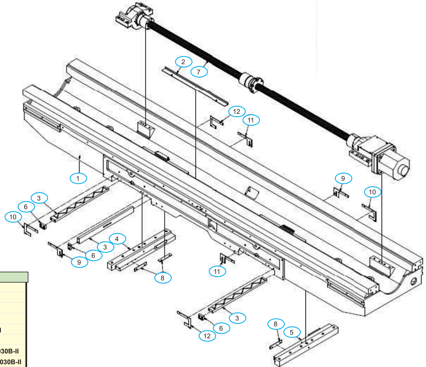
SADDLE CASTING
