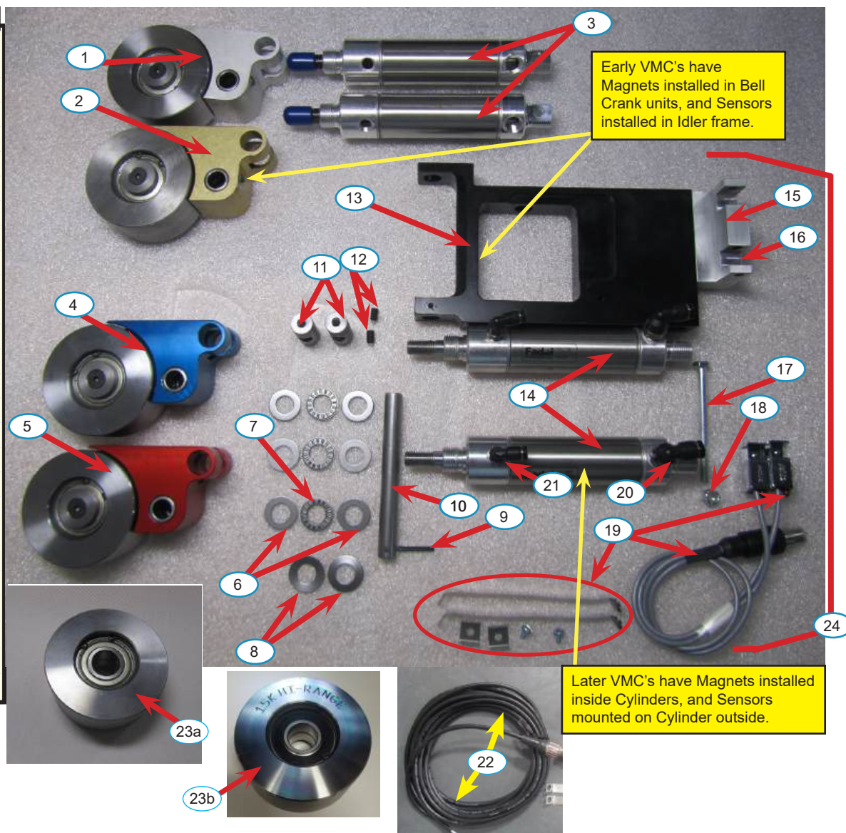
IDLER ASSEMBLY
